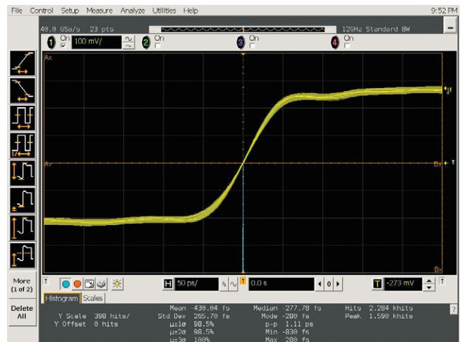
Figure 8. With the industry's lowest trigger jitter – less than 500 fs rms (typically, less than 200 fs rms on 5 Gb/s PRBS signal) – the DSA80000B facilitates accurate waveform viewing of multiple waveforms.
